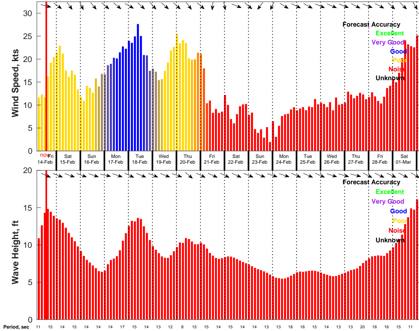
Wind & Wave Forecast for NDBC 46053 from 14-Feb-2025 05:00:00 to 02-Mar-2025 05:00:00
