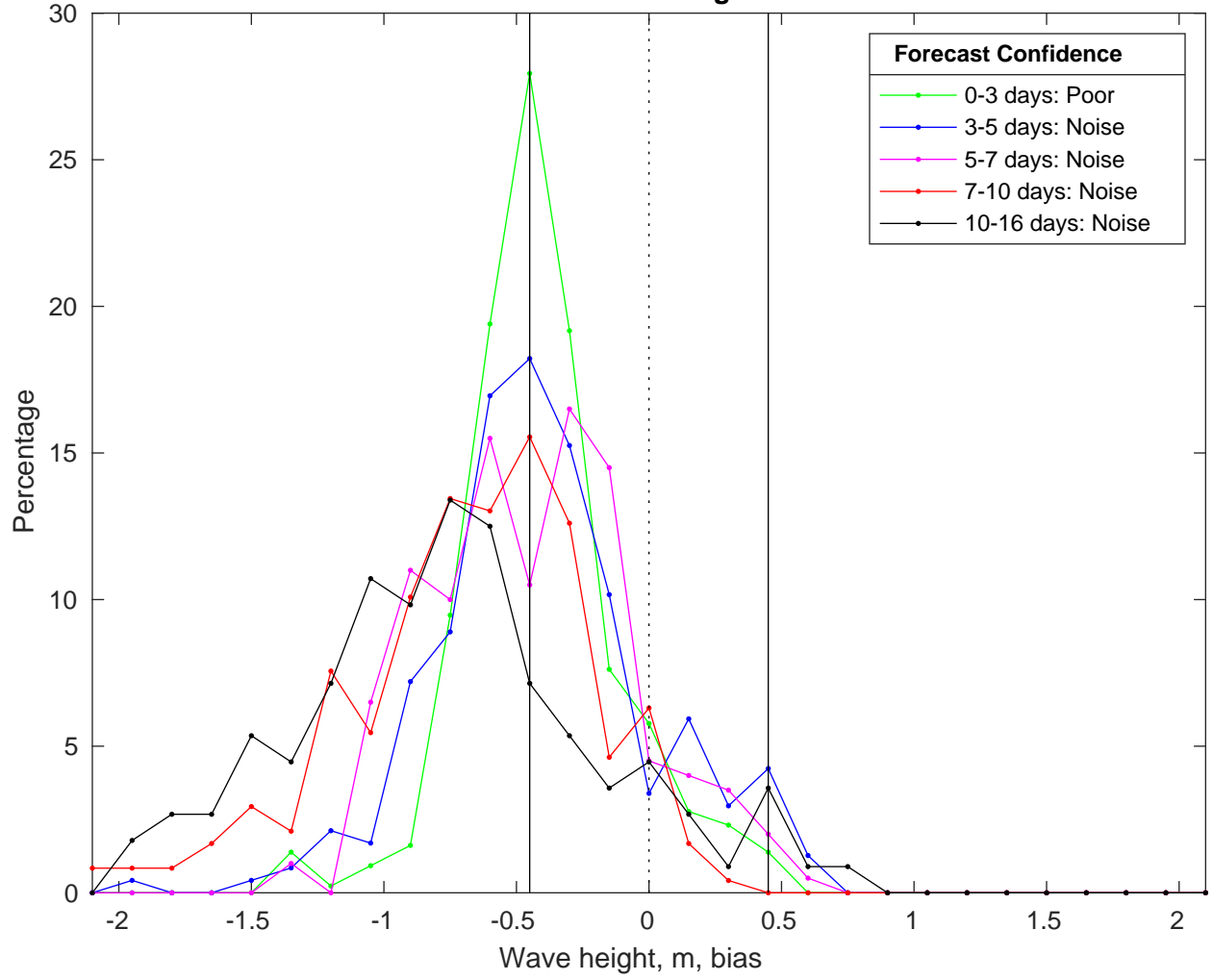
NDBC 46054 vs GFS Waves Bias Histogram: 14-Feb-2025
