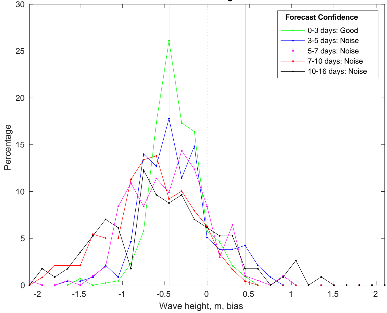
NDBC 46069 vs GFS Waves Bias Histogram: 14-Feb-2025
