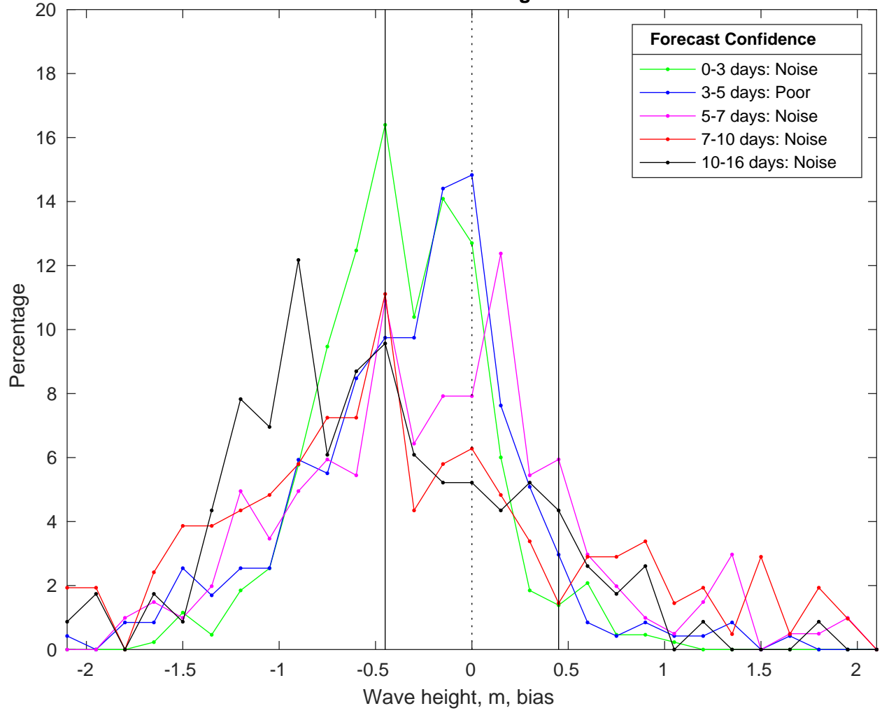
NDBC 46246 vs GFS Waves Bias Histogram: 14-Feb-2025
