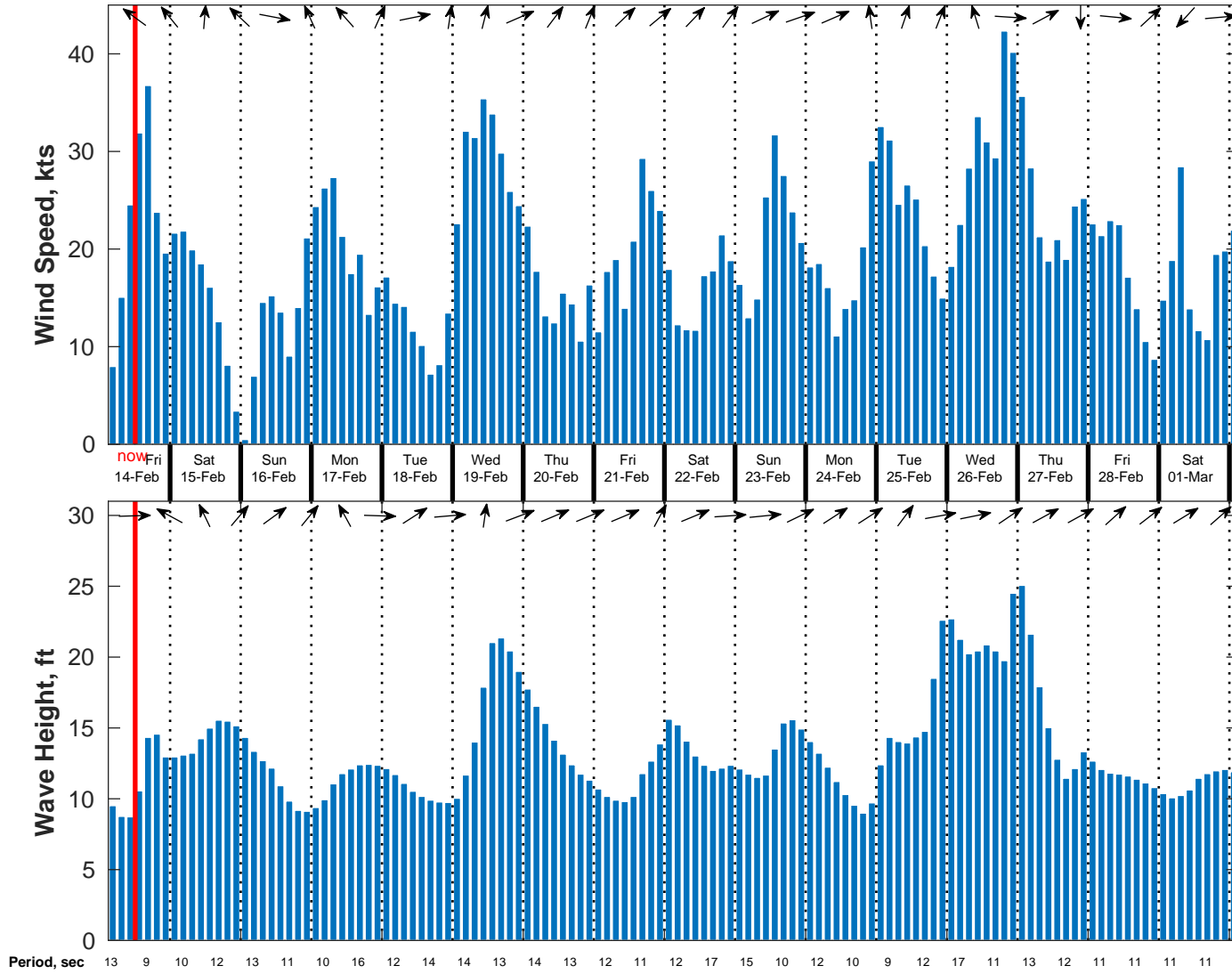
Wind & Wave Forecast for NDBC 46246 from 14-Feb-2025 03:00:00 to 02-Mar-2025 03:00:00
