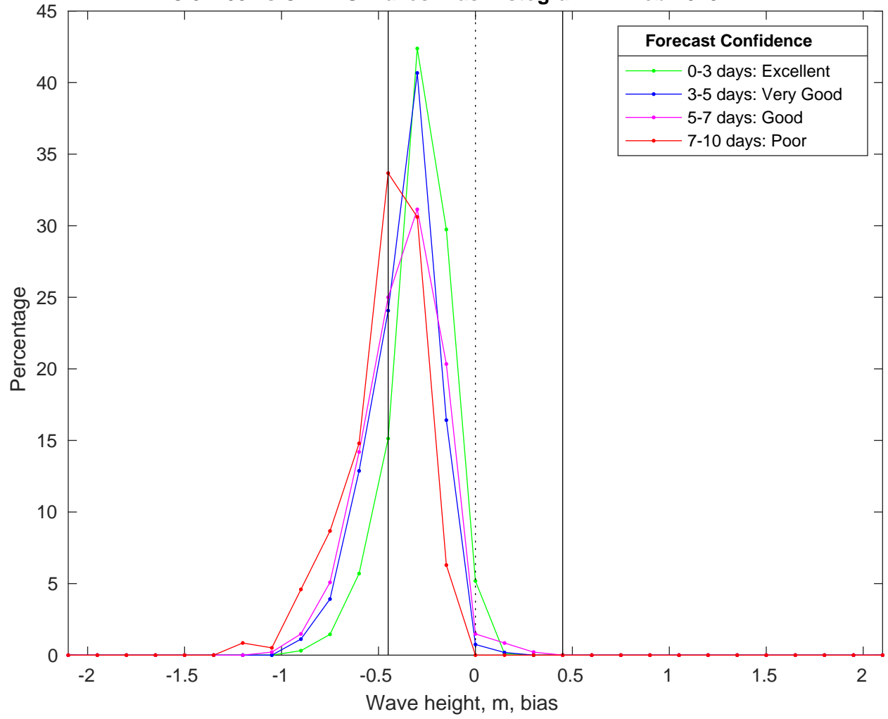
NDBC 51209 vs CMEMS Waves Bias Histogram: 14-Feb-2025
