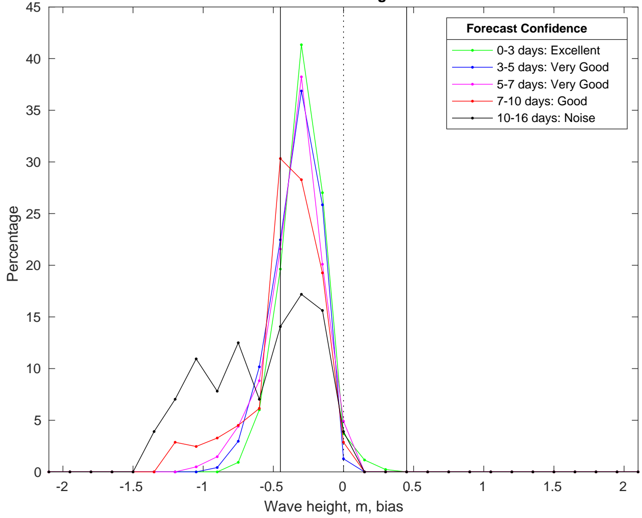
NDBC 51209 vs GFS Waves Bias Histogram: 14-Feb-2025
