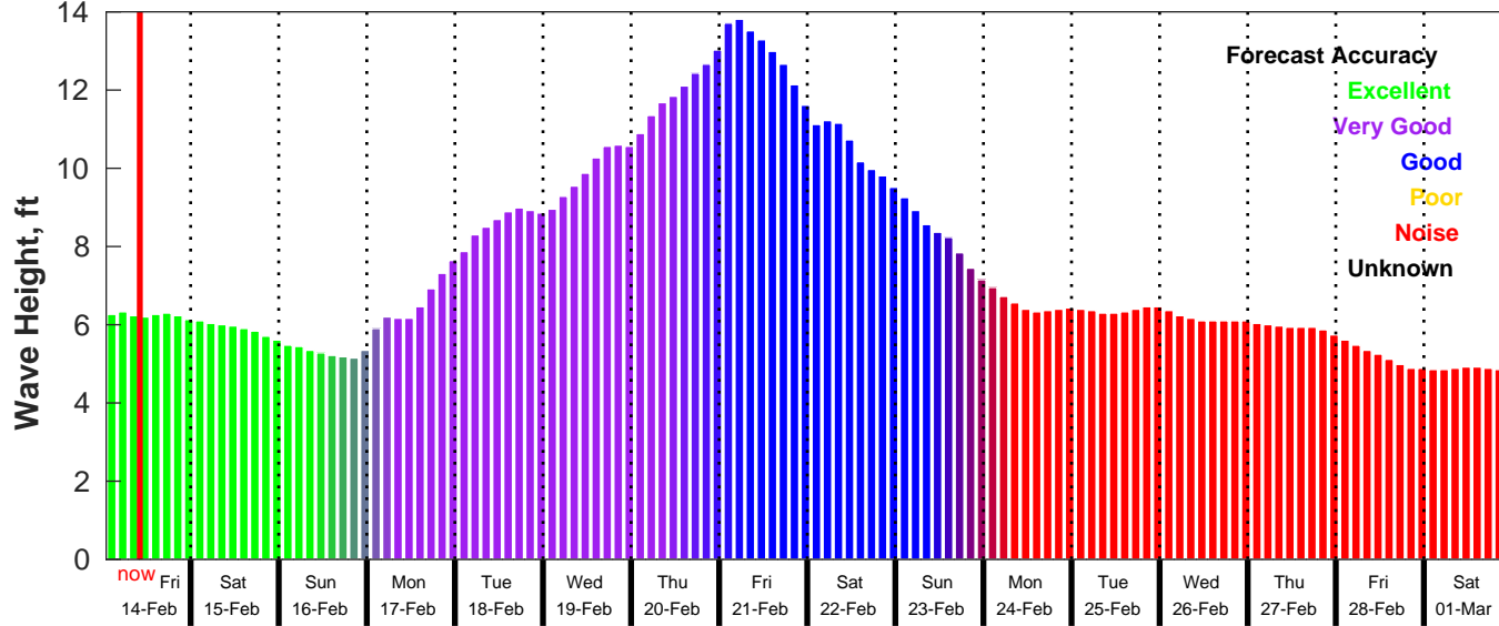
GFS Wave Forecast for NDBC 51209 from 14-Feb-2025 01:00:00 to 02-Mar-2025 01:00:00
