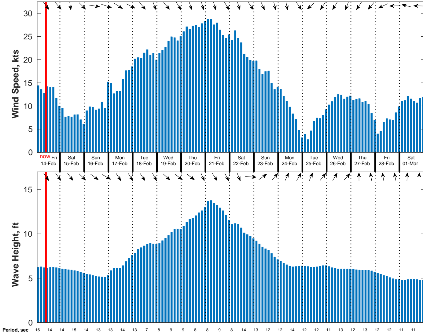
Wind & Wave Forecast for NDBC 51209 from 14-Feb-2025 01:00:00 to 02-Mar-2025 01:00:00
