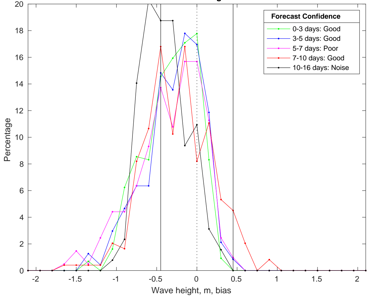
NDBC 52211 vs GFS Waves Bias Histogram: 14-Feb-2025
