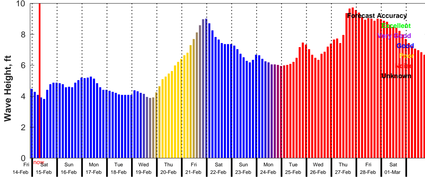
GFS Wave Forecast for NDBC 52211 from 14-Feb-2025 22:00:00 to 02-Mar-2025 22:00:00
