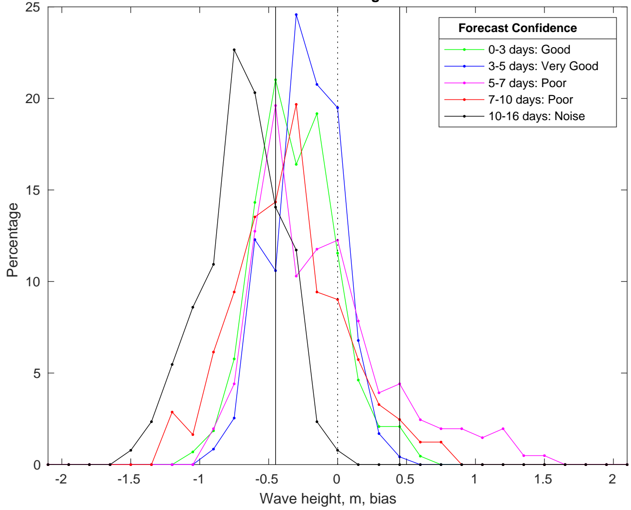
NDBC 52212 vs GFS Waves Bias Histogram: 14-Feb-2025
