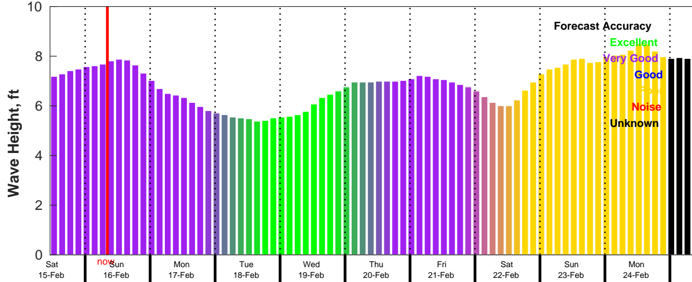
CMEMS Wave Forecast for NDBC 52213 from 14-Feb-2025 11:00:00 to 24-Feb-2025 11:00:00
