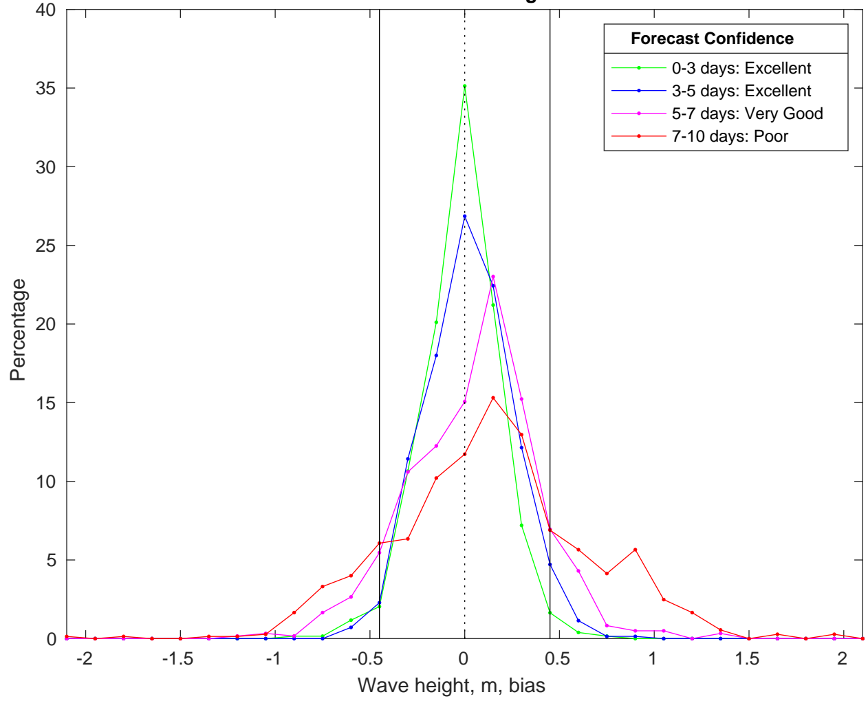
NDBC 41004 vs CMEMS Waves Bias Histogram: 15-Feb-2025
