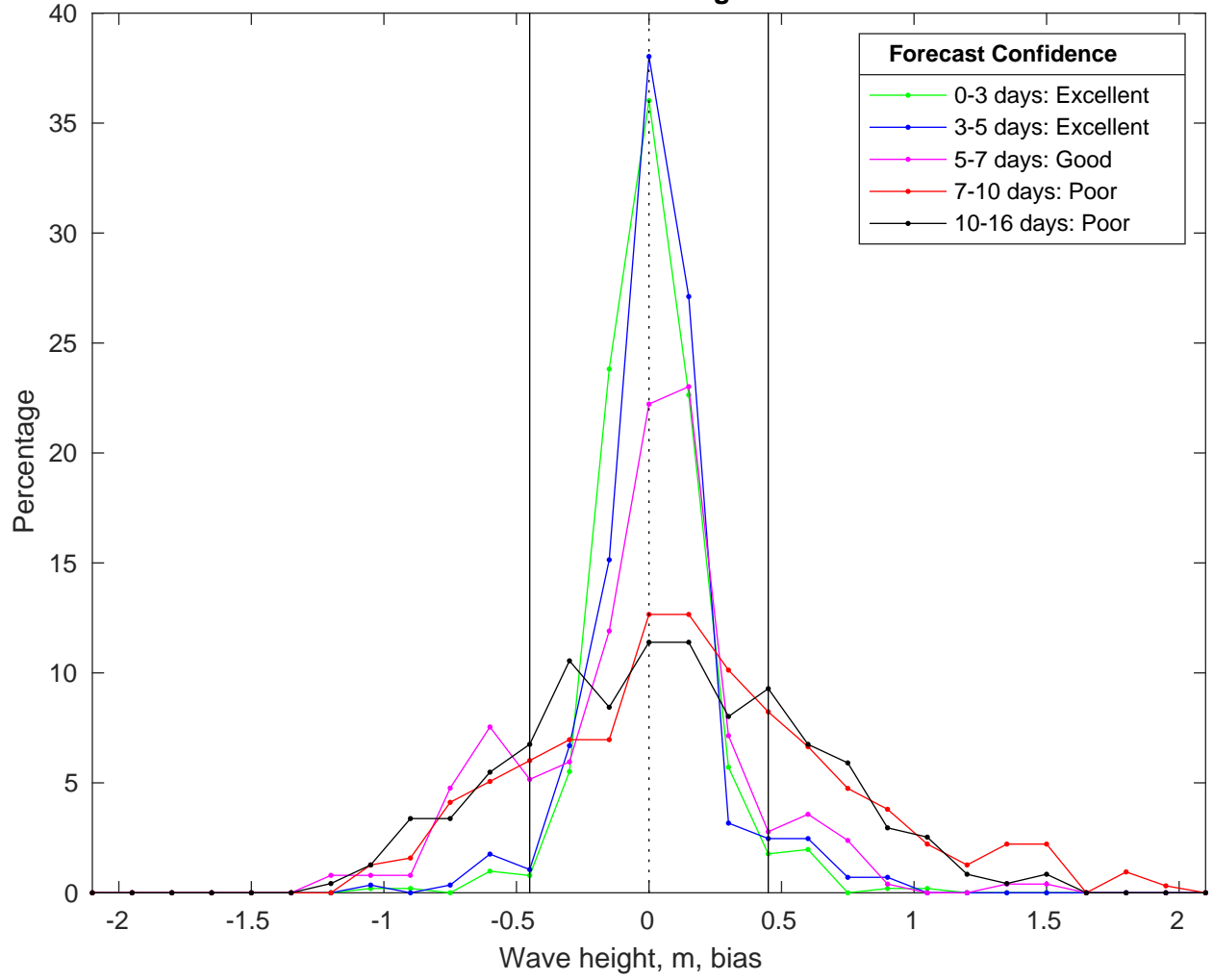
NDBC 41004 vs GFS Waves Bias Histogram: 15-Feb-2025
