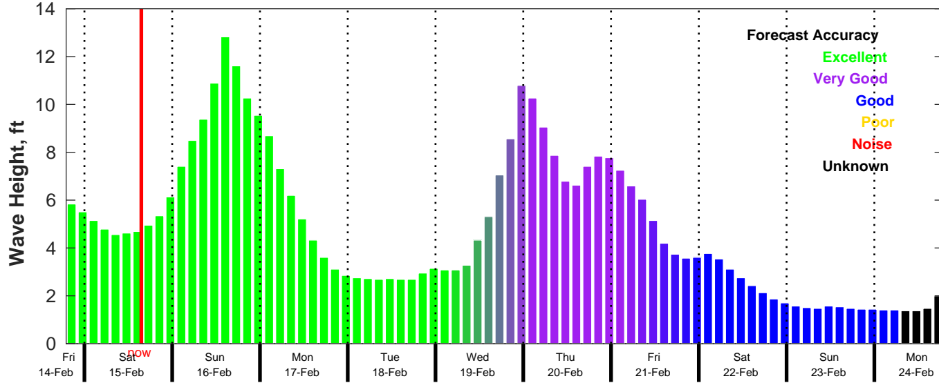
CMEMS Wave Forecast for NDBC 41013 from 14-Feb-2025 19:00:00 to 24-Feb-2025 19:00:00
