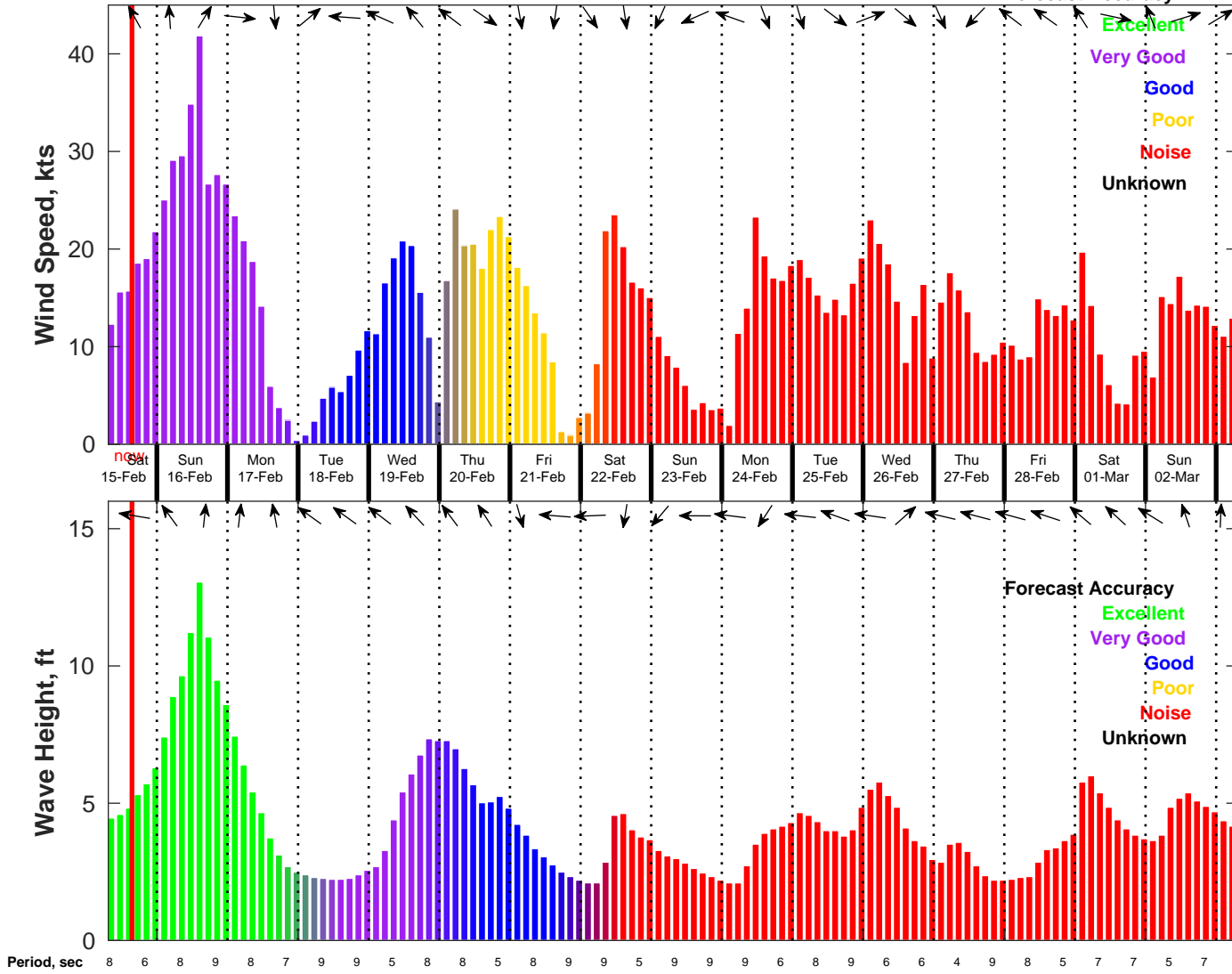
Wind & Wave Forecast for NDBC 41013 from 15-Feb-2025 07:00:00 to 03-Mar-2025 07:00:00
