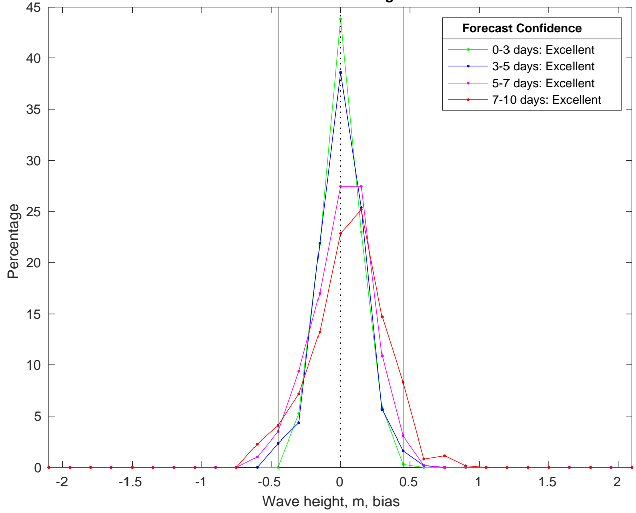
NDBC 41040 vs CMEMS Waves Bias Histogram: 15-Feb-2025
