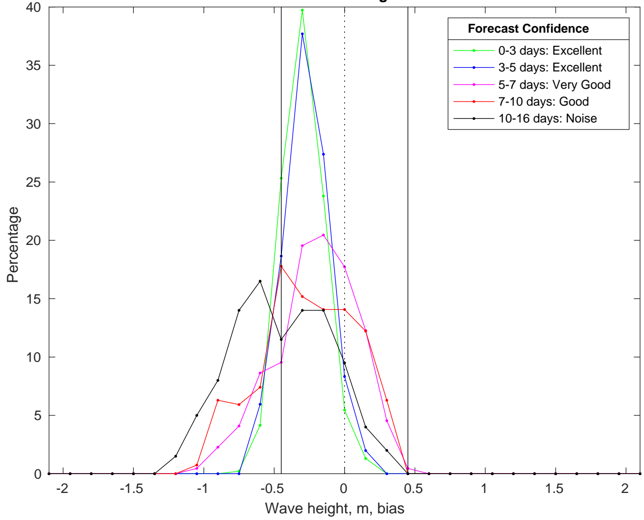
NDBC 41040 vs GFS Waves Bias Histogram: 15-Feb-2025
