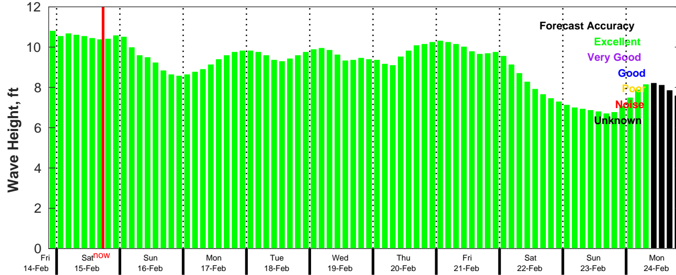
CMEMS Wave Forecast for NDBC 41040 from 14-Feb-2025 21:00:00 to 24-Feb-2025 21:00:00
