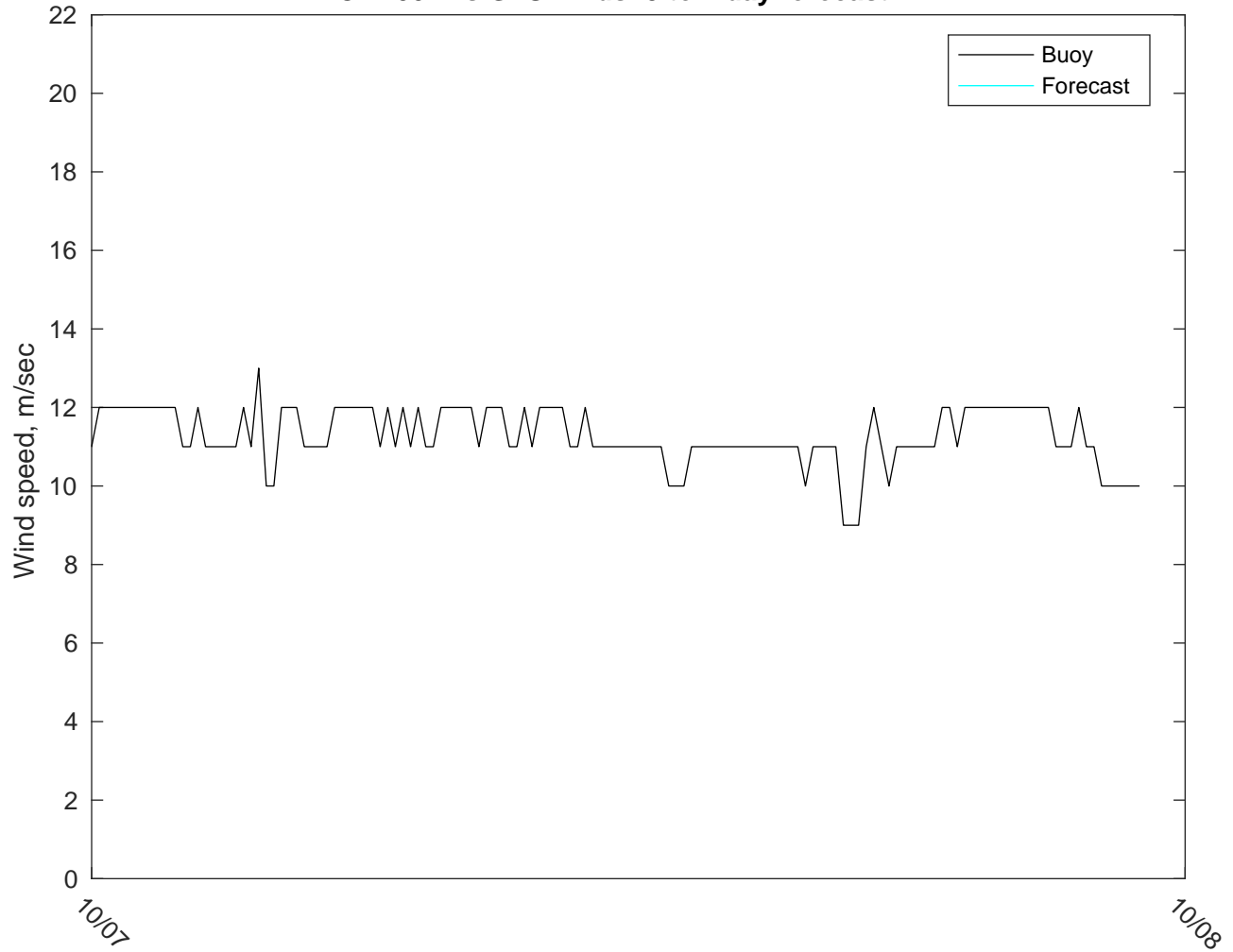
NDBC 42002 vs GFSWinds: 5 to 7 day forecast
