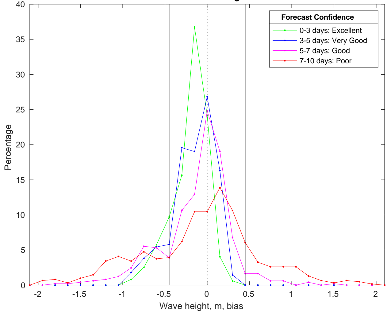
NDBC 42019 vs CMEMS Waves Bias Histogram: 15-Feb-2025
