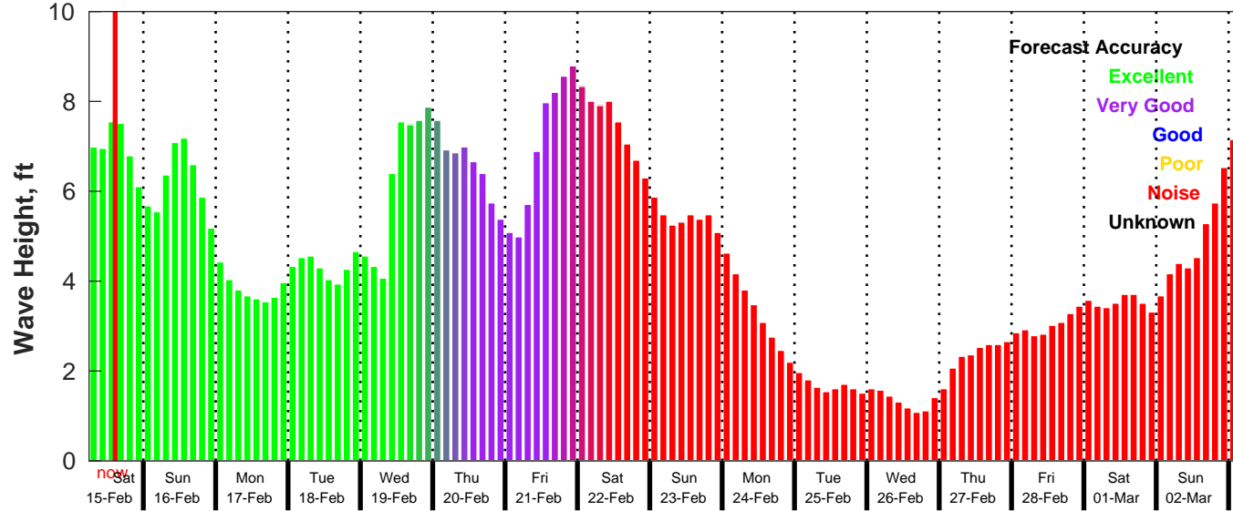
GFS Wave Forecast for NDBC 42019 from 15-Feb-2025 06:00:00 to 03-Mar-2025 06:00:00
