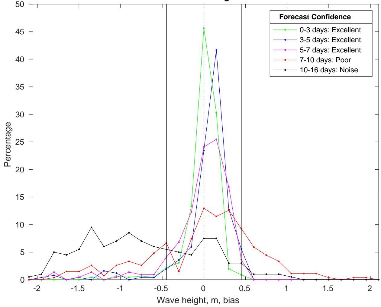
NDBC 42020 vs GFS Waves Bias Histogram: 15-Feb-2025
