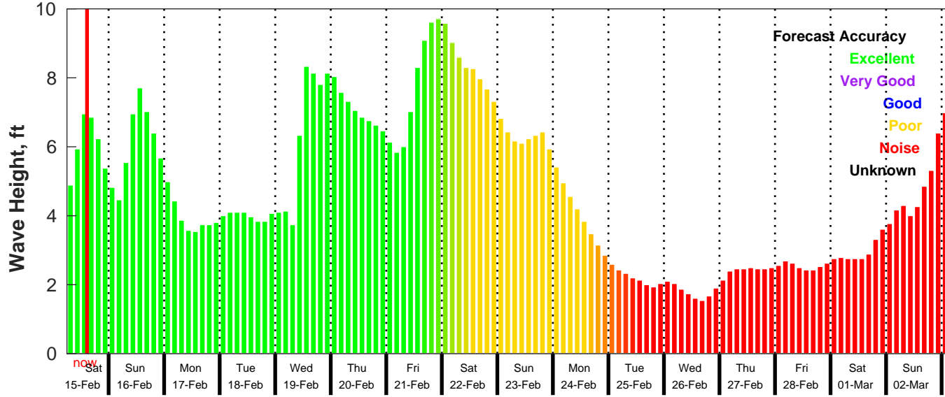
GFS Wave Forecast for NDBC 42020 from 15-Feb-2025 06:00:00 to 03-Mar-2025 06:00:00
