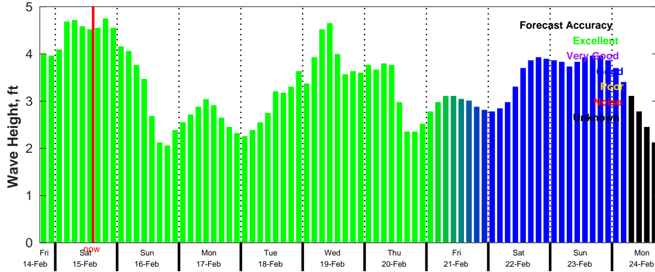
CMEMS Wave Forecast for NDBC 42035 from 14-Feb-2025 18:00:00 to 24-Feb-2025 18:00:00
