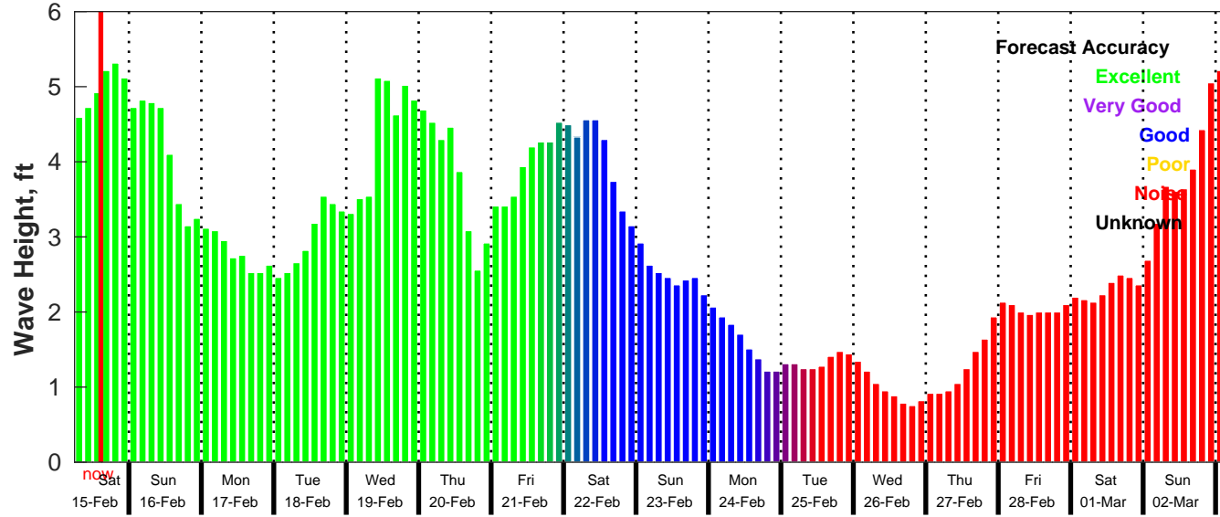
GFS Wave Forecast for NDBC 42035 from 15-Feb-2025 06:00:00 to 03-Mar-2025 06:00:00
