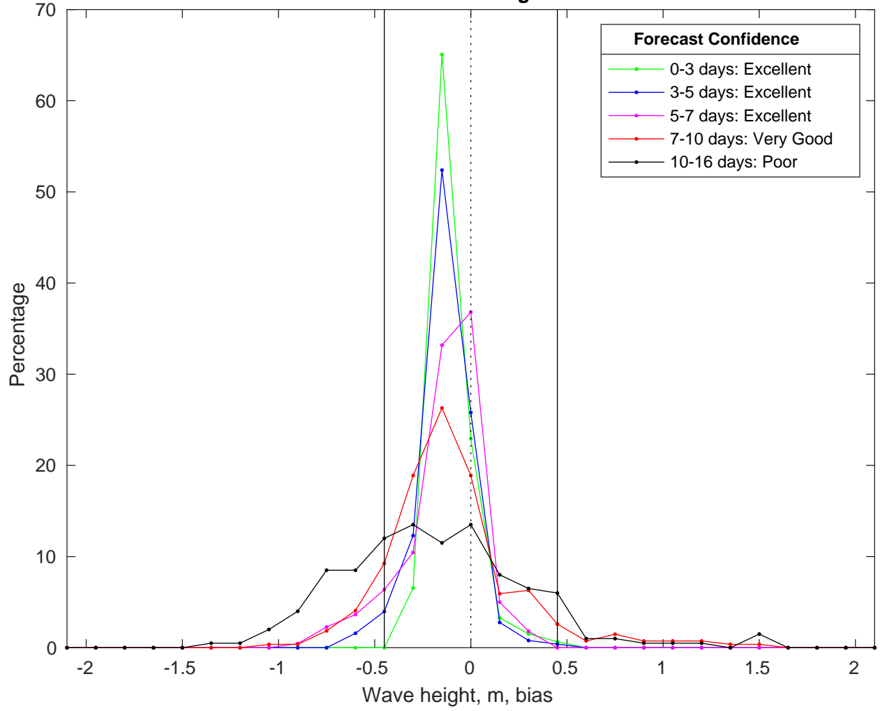
NDBC 42036 vs GFS Waves Bias Histogram: 15-Feb-2025
