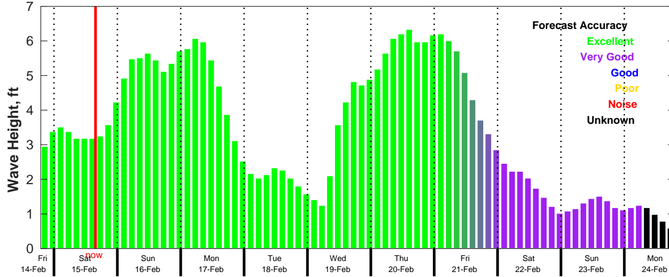
CMEMS Wave Forecast for NDBC 42036 from 14-Feb-2025 19:00:00 to 24-Feb-2025 19:00:00
