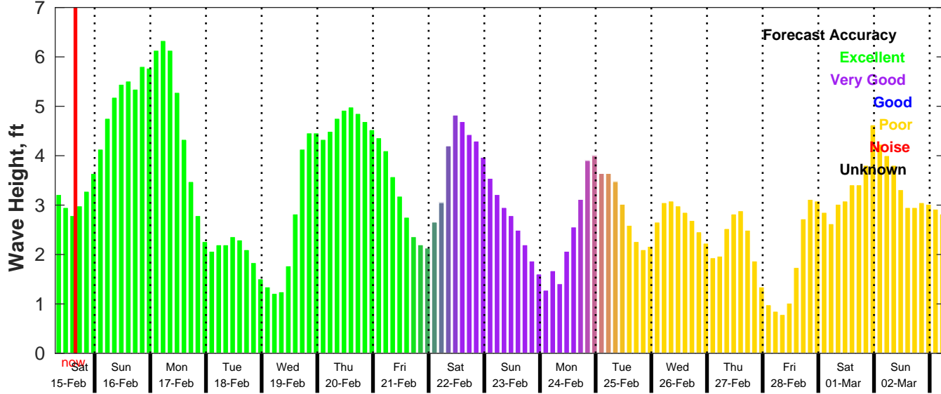
GFS Wave Forecast for NDBC 42036 from 15-Feb-2025 07:00:00 to 03-Mar-2025 07:00:00
