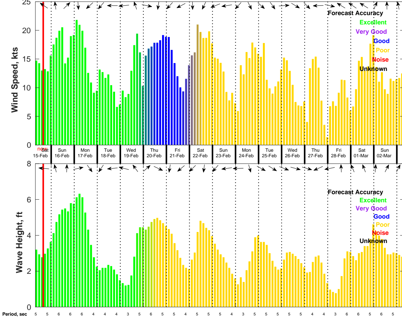
Wind & Wave Forecast for NDBC 42036 from 15-Feb-2025 07:00:00 to 03-Mar-2025 07:00:00
