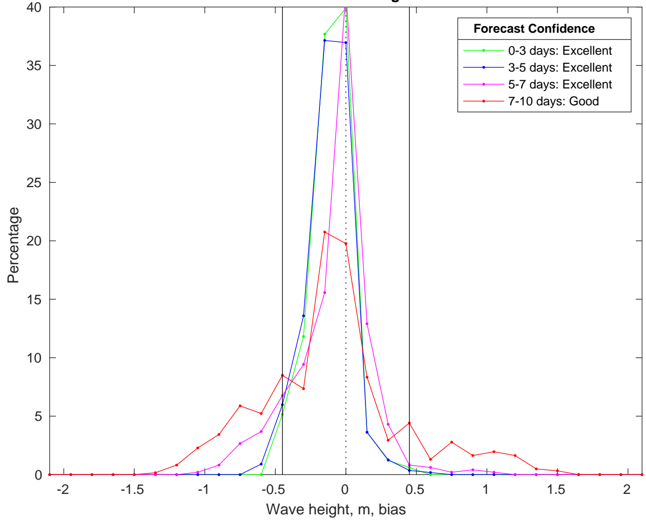
NDBC 42040 vs CMEMS Waves Bias Histogram: 15-Feb-2025
