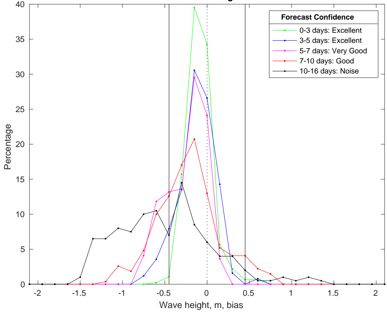
NDBC 42040 vs GFS Waves Bias Histogram: 15-Feb-2025
