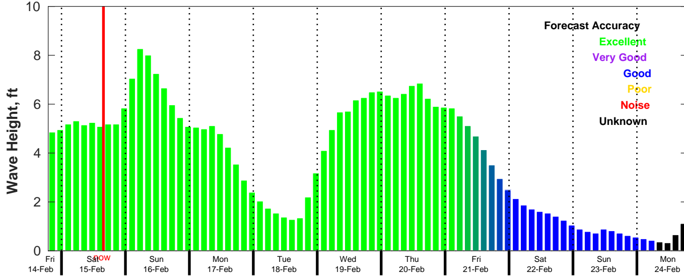
CMEMS Wave Forecast for NDBC 42040 from 14-Feb-2025 19:00:00 to 24-Feb-2025 19:00:00
