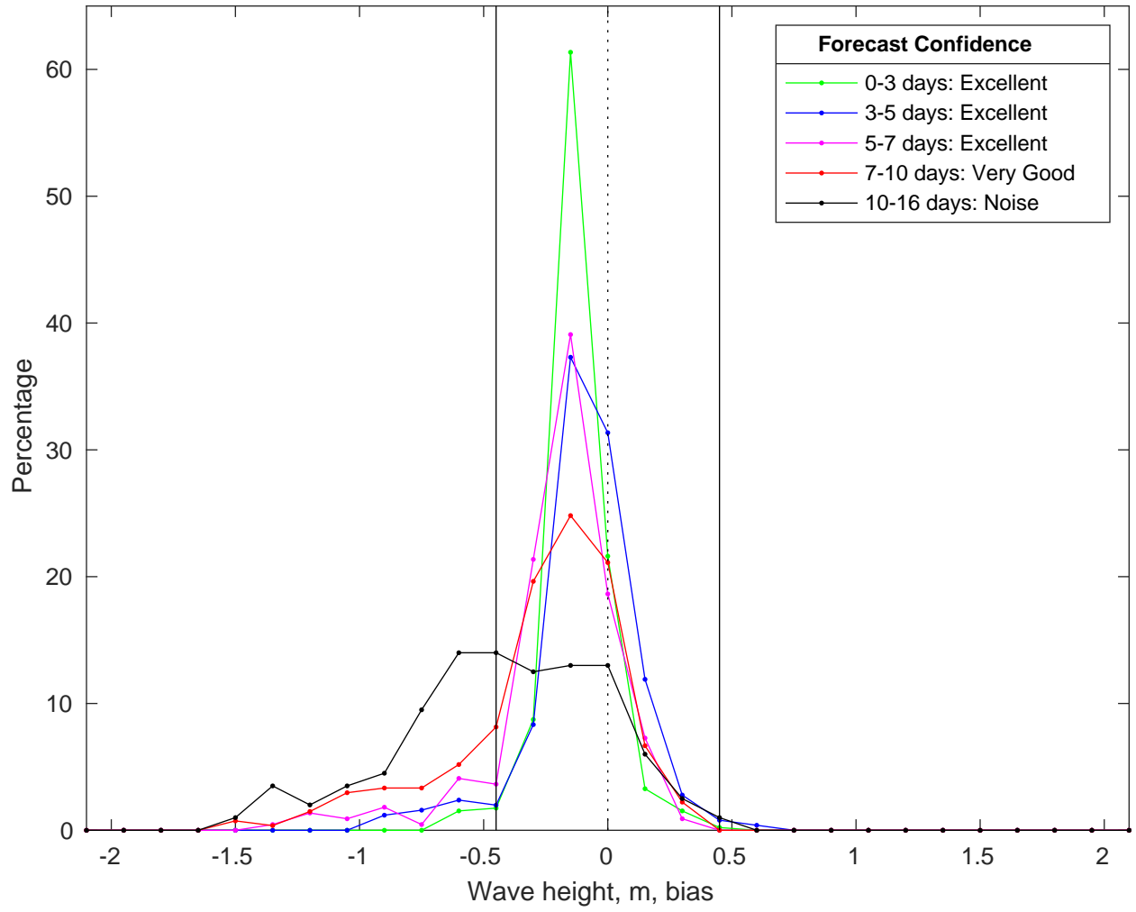
NDBC 42084 vs GFS Waves Bias Histogram: 15-Feb-2025
