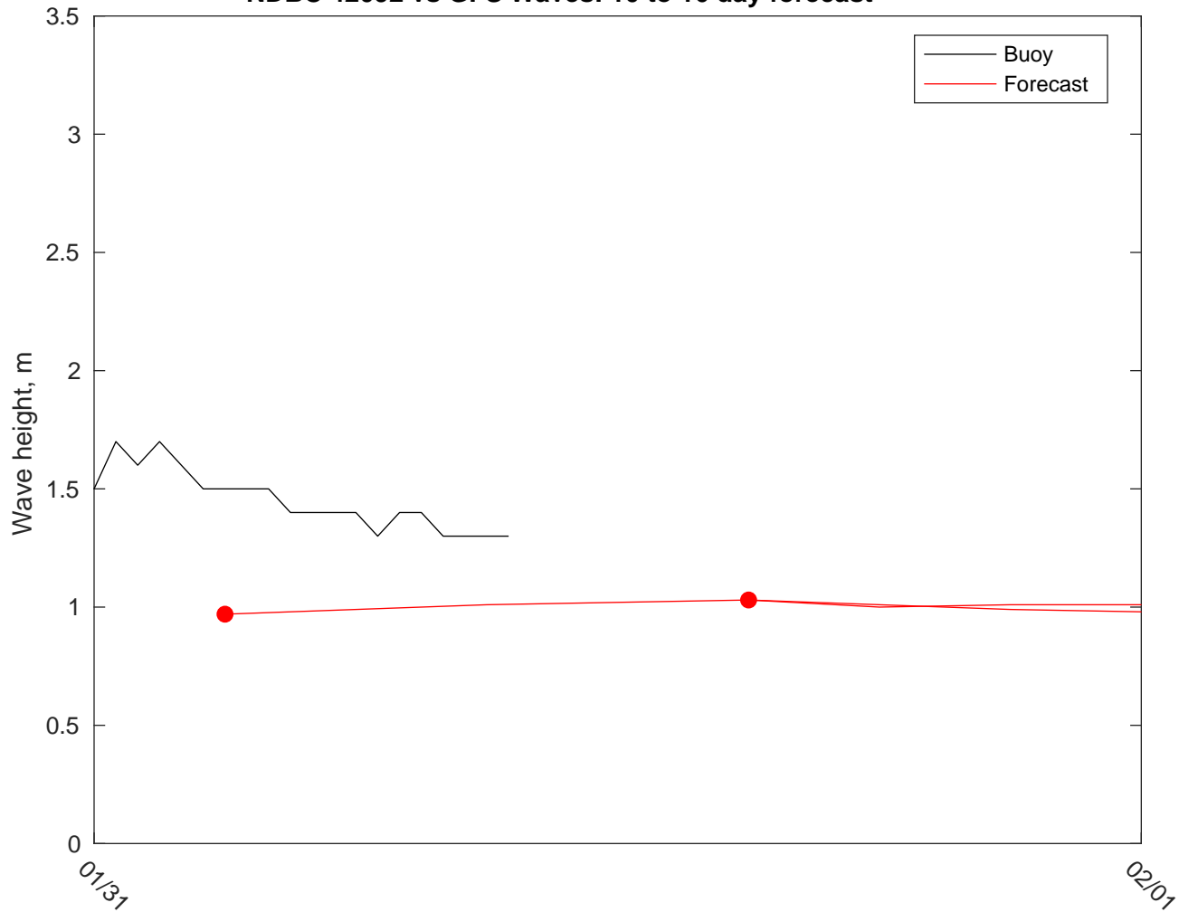
NDBC 42092 vs GFS Waves: 10 to 16 day forecast
