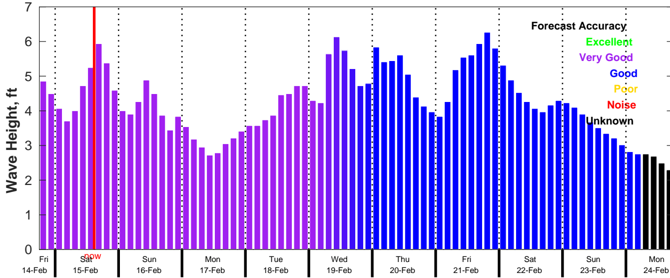
CMEMS Wave Forecast for NDBC 42092 from 14-Feb-2025 18:00:00 to 24-Feb-2025 18:00:00
