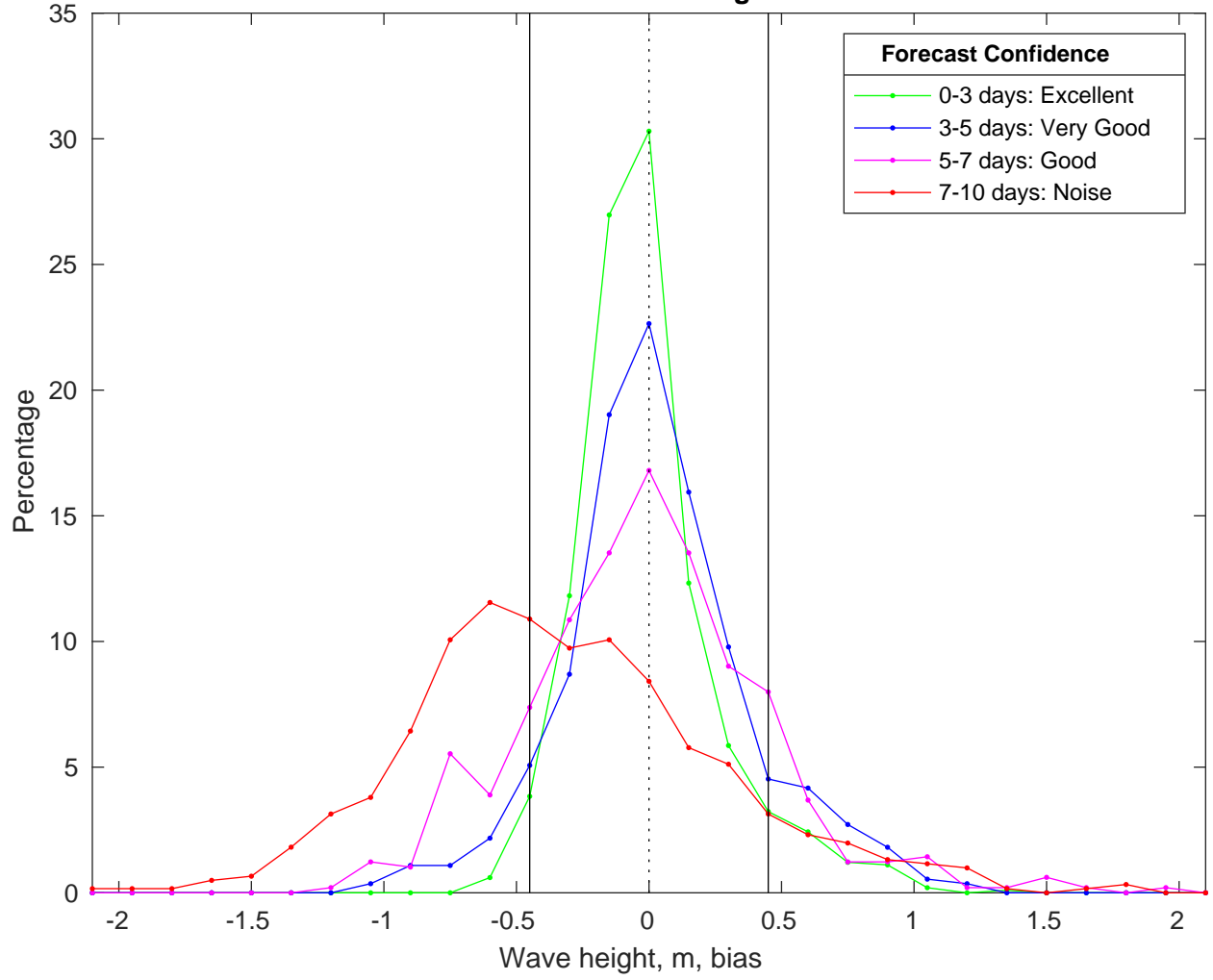
NDBC 46011 vs CMEMS Waves Bias Histogram: 15-Feb-2025
