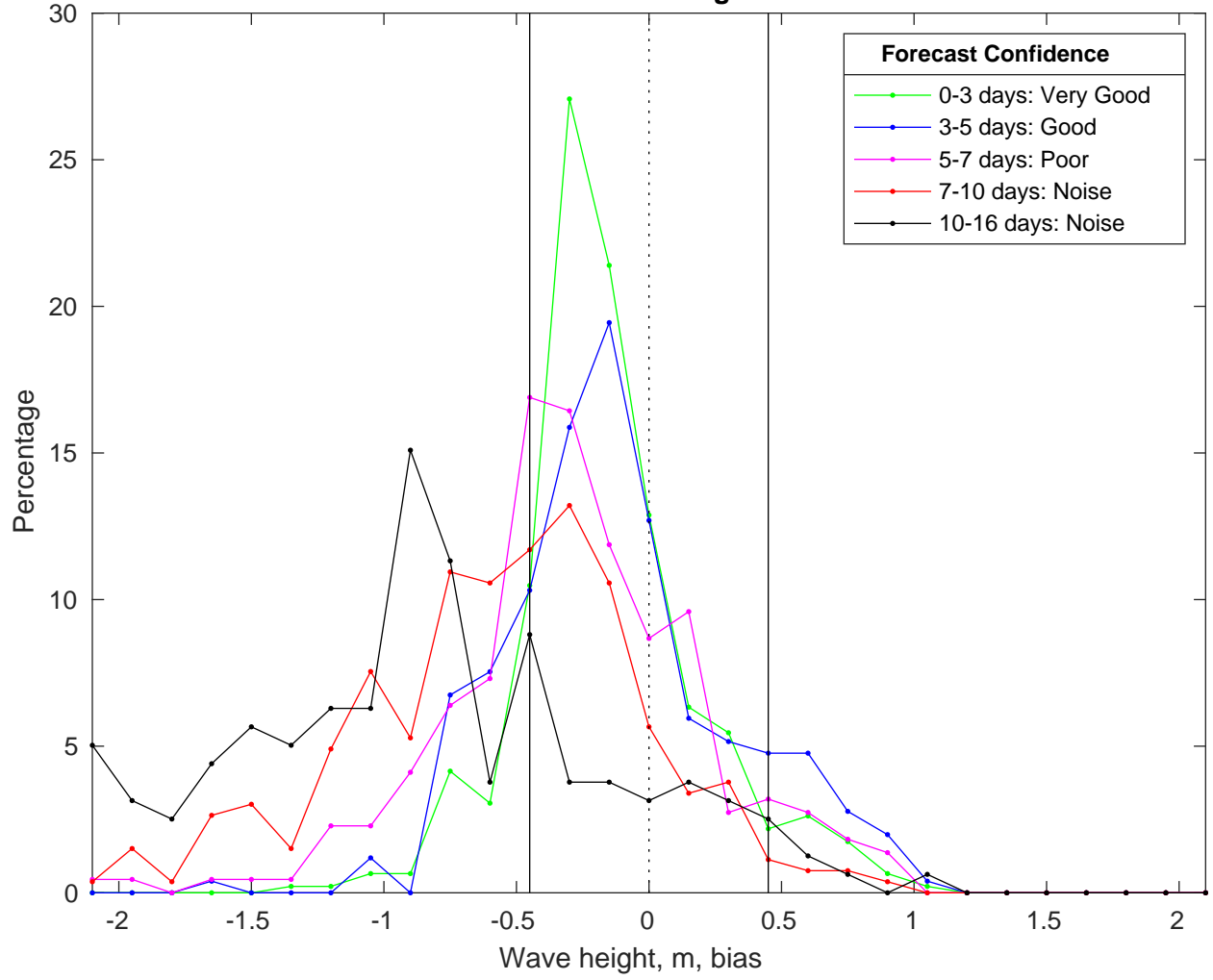
NDBC 46011 vs GFS Waves Bias Histogram: 15-Feb-2025
