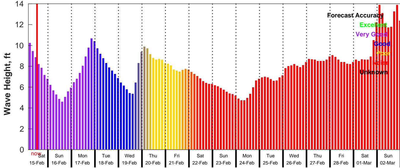
GFS Wave Forecast for NDBC 46011 from 15-Feb-2025 04:00:00 to 03-Mar-2025 04:00:00
