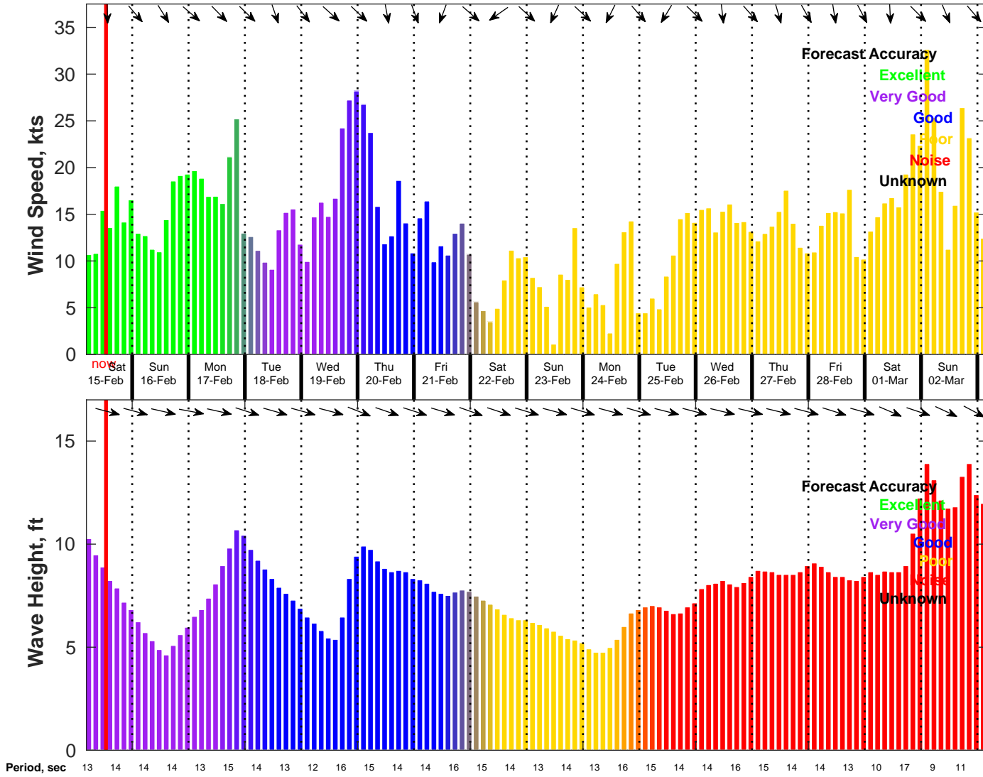
Wind & Wave Forecast for NDBC 46011 from 15-Feb-2025 04:00:00 to 03-Mar-2025 04:00:00
