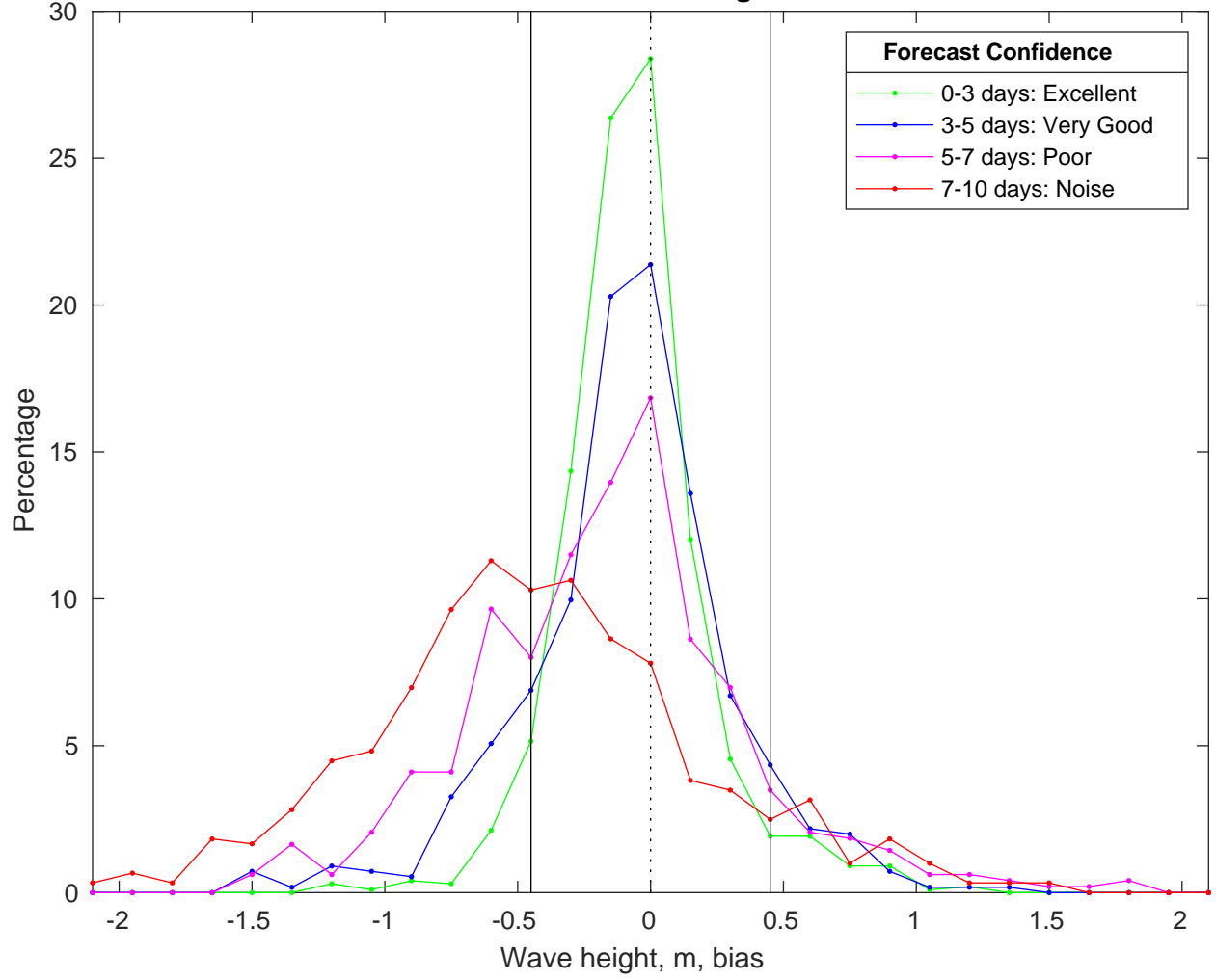
NDBC 46028 vs CMEMS Waves Bias Histogram: 15-Feb-2025
