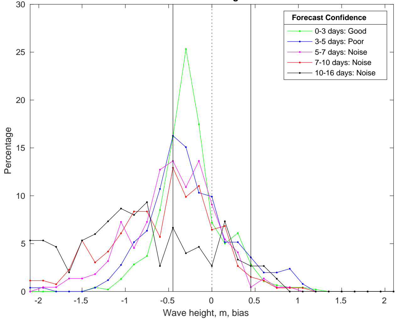
NDBC 46028 vs GFS Waves Bias Histogram: 15-Feb-2025
