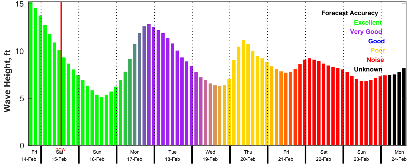
CMEMS Wave Forecast for NDBC 46028 from 14-Feb-2025 16:00:00 to 24-Feb-2025 16:00:00
