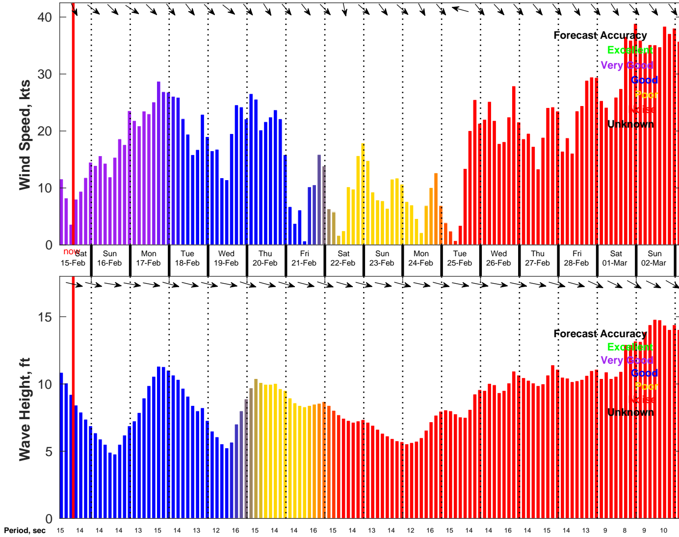
Wind & Wave Forecast for NDBC 46028 from 15-Feb-2025 04:00:00 to 03-Mar-2025 04:00:00
