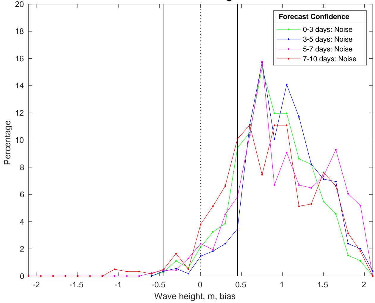
NDBC 46053 vs CMEMS Waves Bias Histogram: 15-Feb-2025
