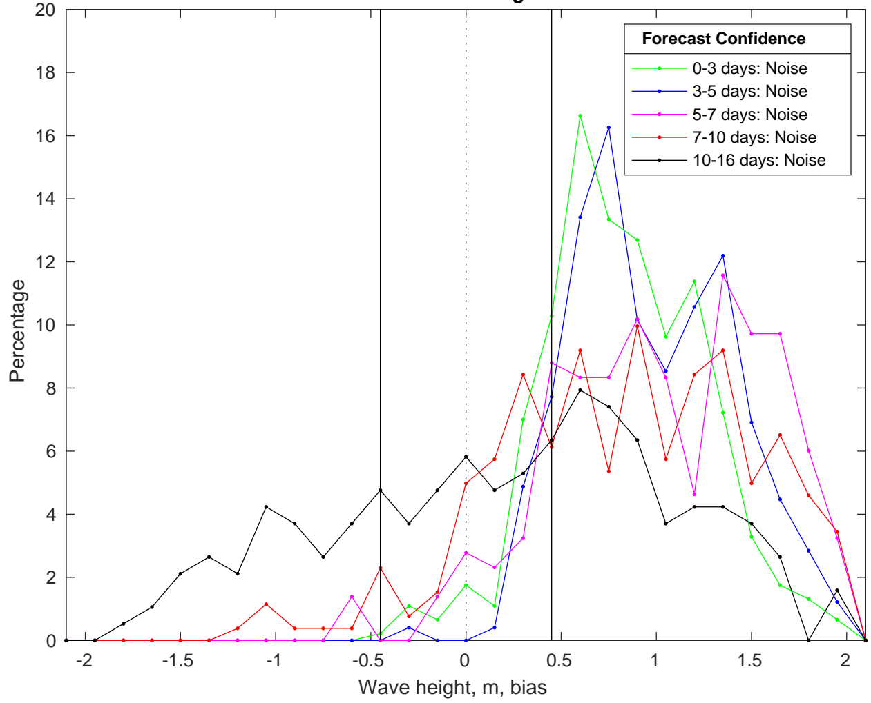
NDBC 46053 vs GFS Waves Bias Histogram: 15-Feb-2025
