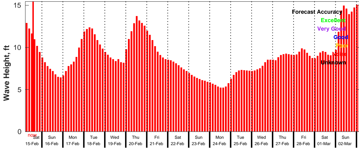
GFS Wave Forecast for NDBC 46053 from 15-Feb-2025 05:00:00 to 03-Mar-2025 05:00:00
