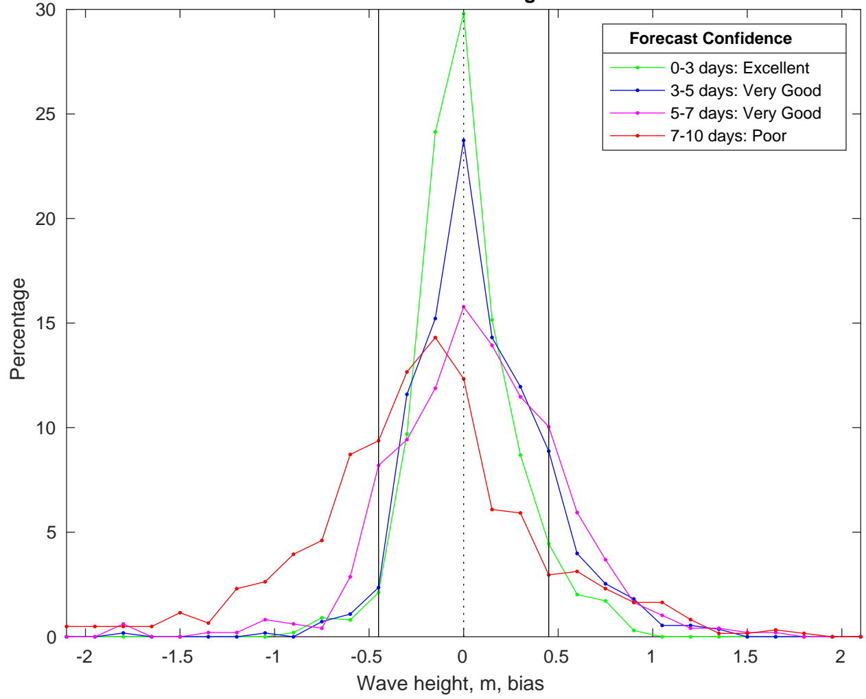
NDBC 46054 vs CMEMS Waves Bias Histogram: 15-Feb-2025
