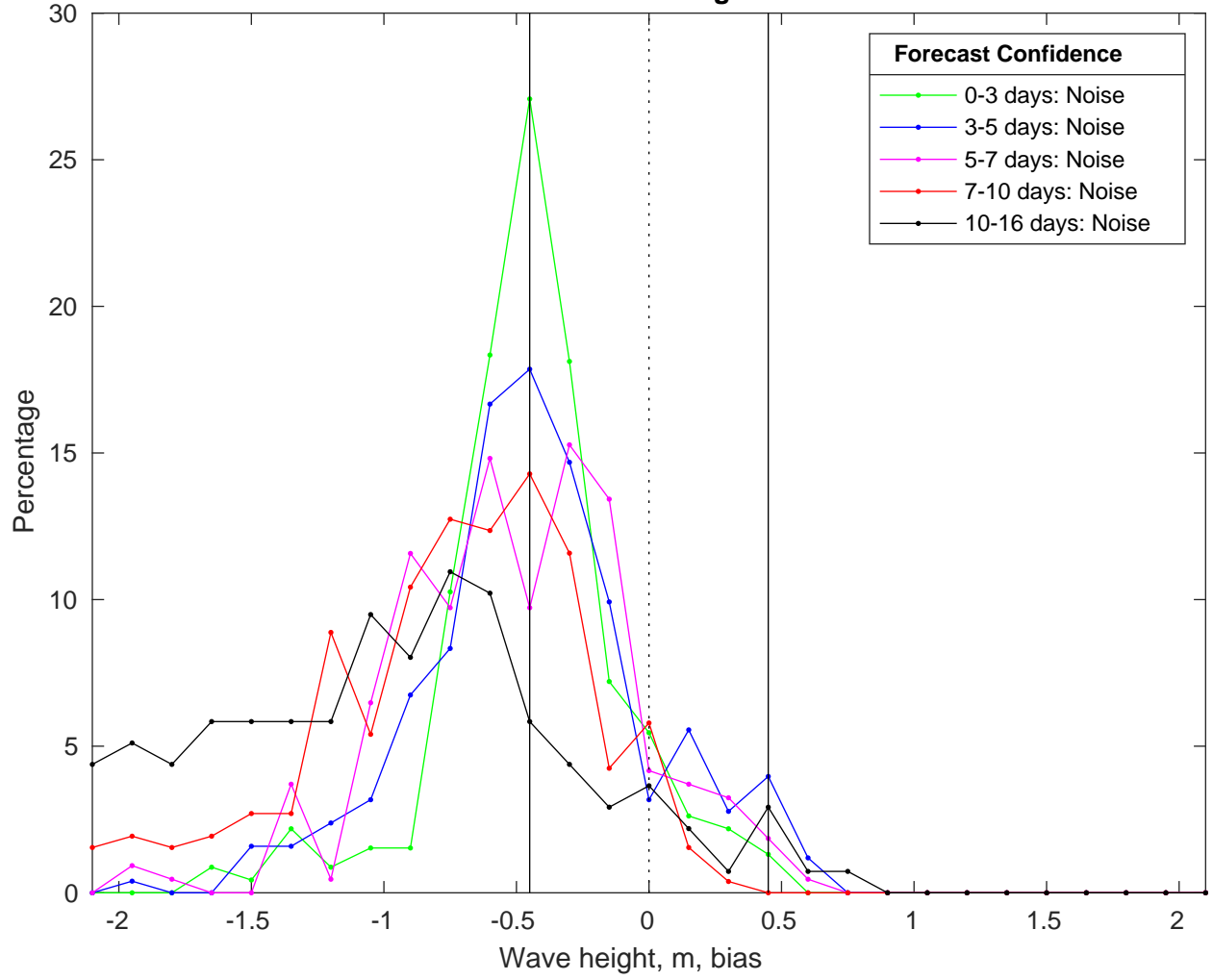
NDBC 46054 vs GFS Waves Bias Histogram: 15-Feb-2025
